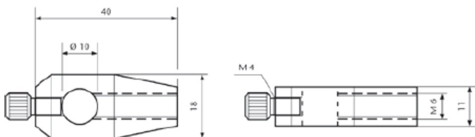
Holder, P/N 158 335
