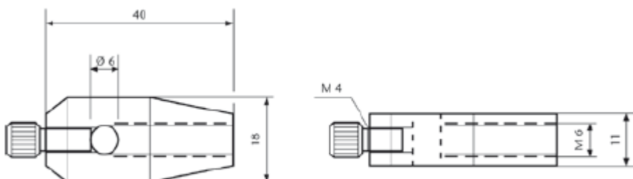
Holder, P/N 158 330
